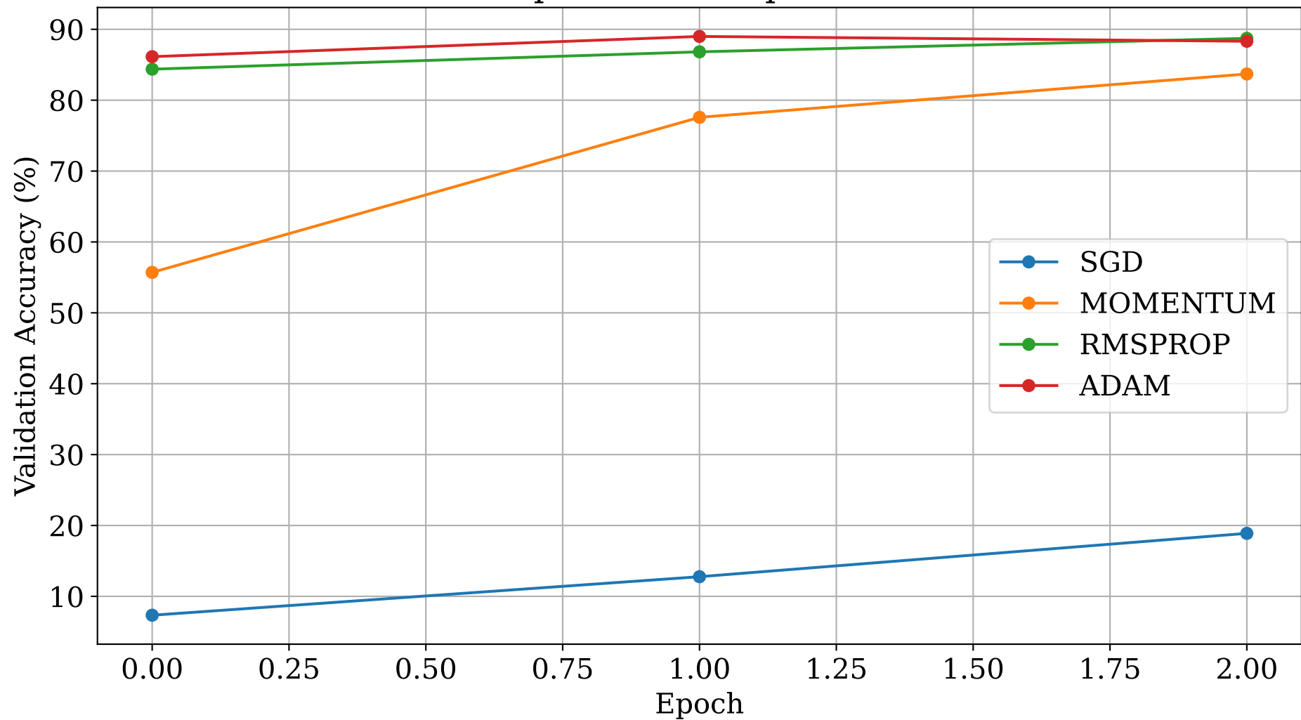
Optimizer Comparison
